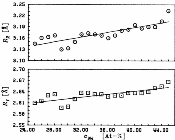
Fig. 4. Amorphous \text{Ni}_x\text{Zr}_{(100-x)} . Atomic distances R_1 (below) and R_2 (above).
