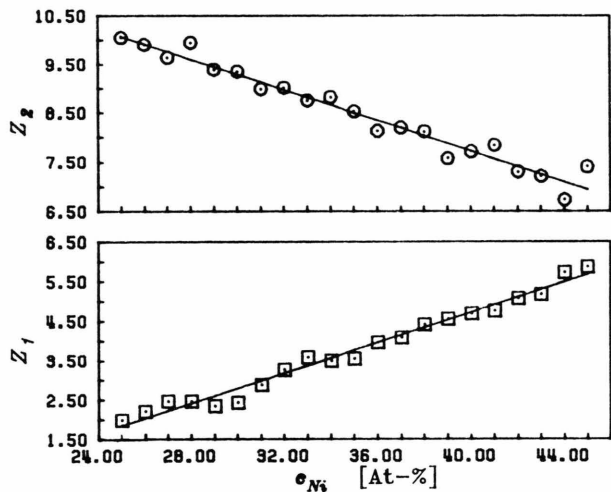
Fig. 5. Amorphous \text{Ni}_x\text{Zr}_{(100-x)} . Coordination numbers Z_1 (below) and Z_2 (above).
